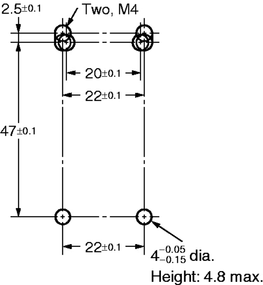
Mounting hole dimensions
